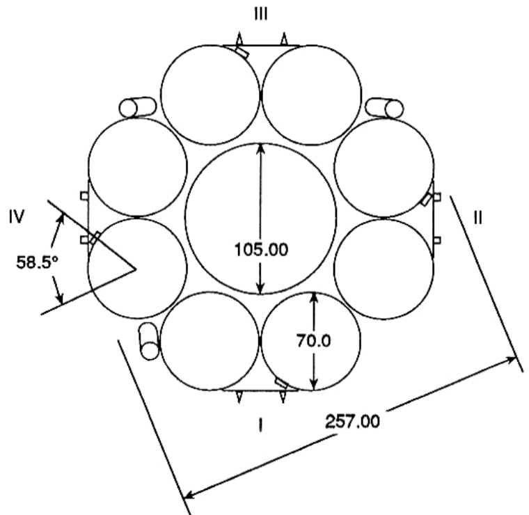
VIEW F-F First stage tanks
