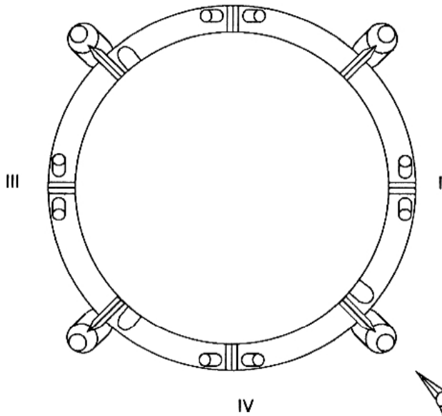
VIEW E-E II Top of first stage
