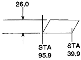
VIEW L-L Turbine exhaust
